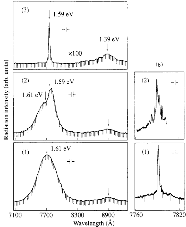
Fig. 1. Radiation spectrum for the first low room-temperature threshold Al x Ga 1-x As DHS laser 300 K. J_{th} = 4300 \text{ A/cm}^2 . Current increases from 0.7 A(1) to 8.3 A(2) and to 13.6 A(3).
